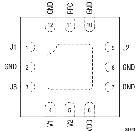
Figure 2. SKY13588-460LF Pinout – 12-Pin QFN (Top View)
