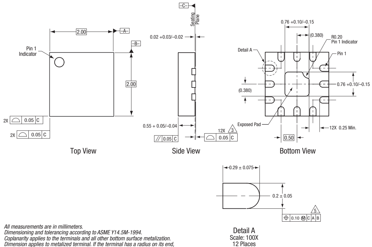
Figure 11. SKY13588-460LF 12-Pin QFN Package Dimensions
