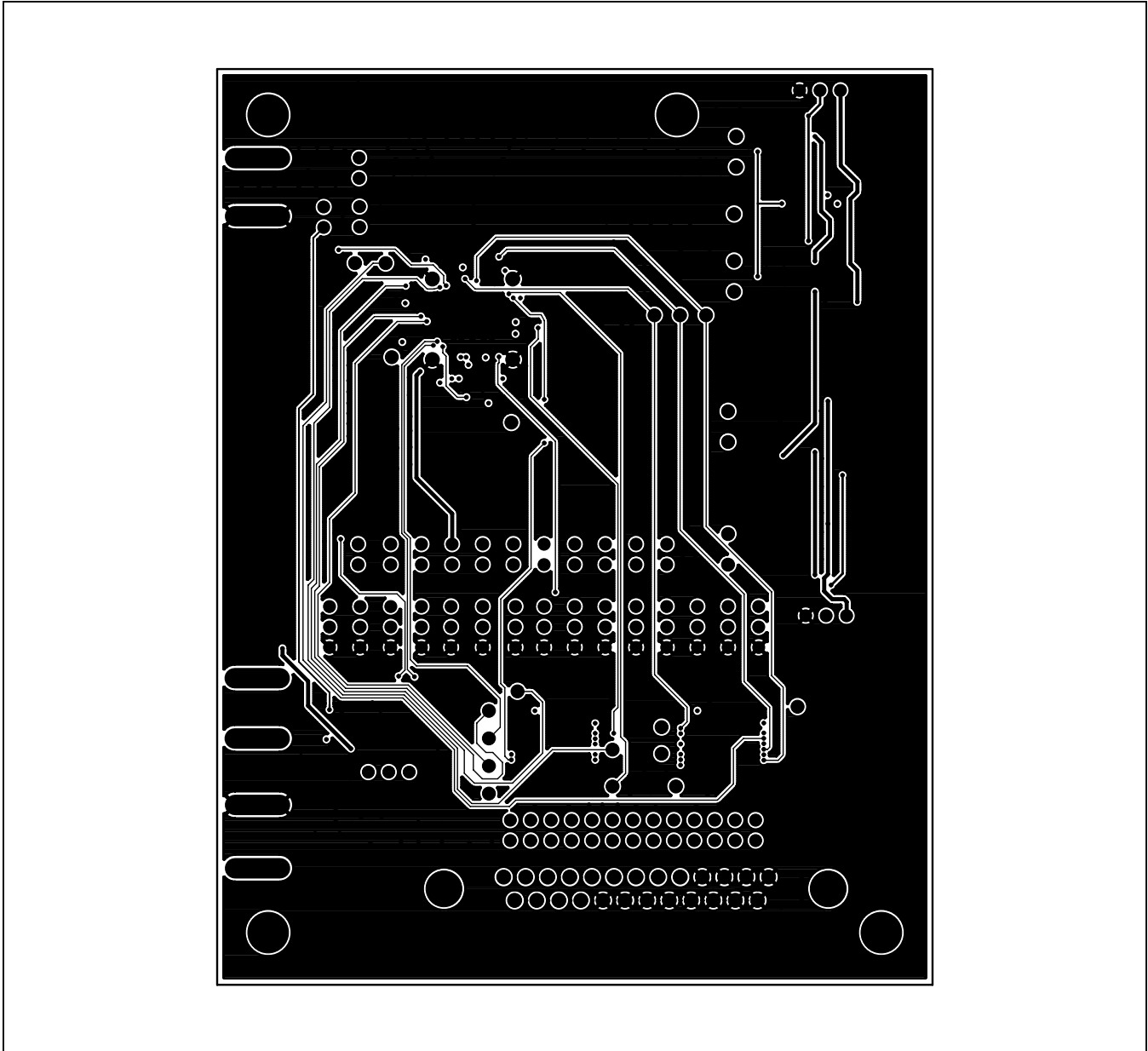
Figure 5. MAX2830 EV Kit PCB Layout—Inner Layer 3 (Routes)
