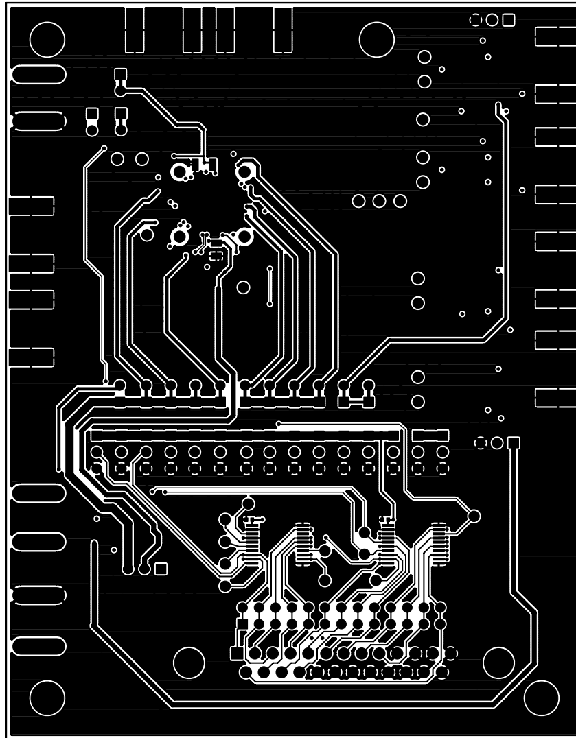
Figure 6. MAX2830 EV Kit PCB Layout—Solder Side
