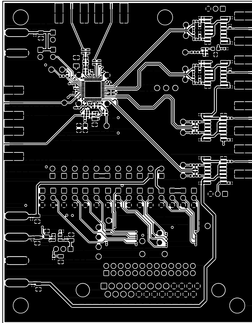
Figure 3. MAX2830 EV Kit PCB Layout—Component Side
