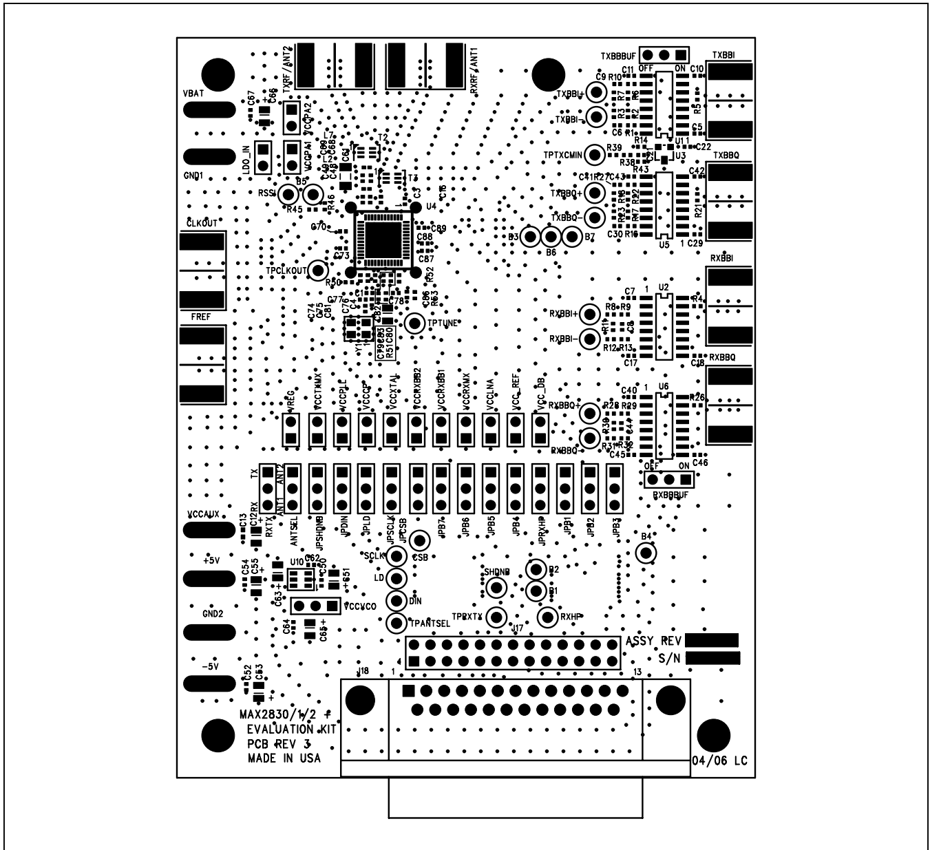
Figure 2. MAX2830 EV Kit PCB Layout—Top Silkscreen
