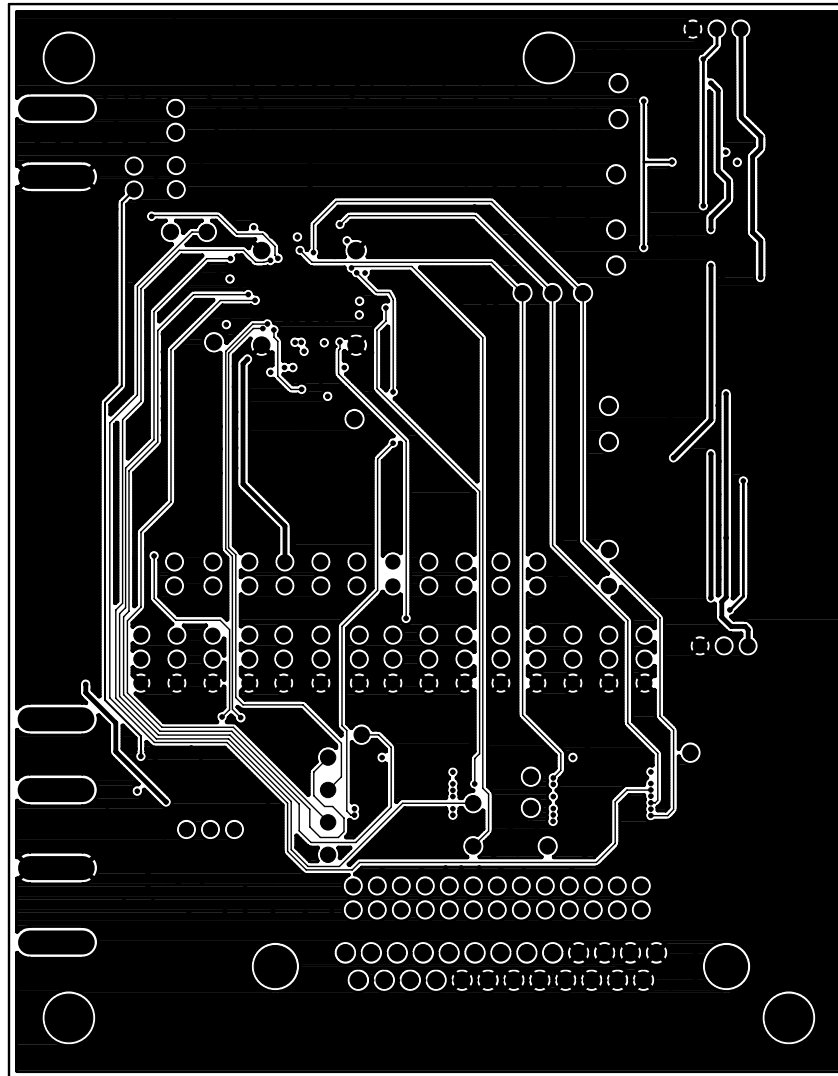
Figure 5. MAX2830 EV Kit PCB Layout—Inner Layer 3 (Routes)
