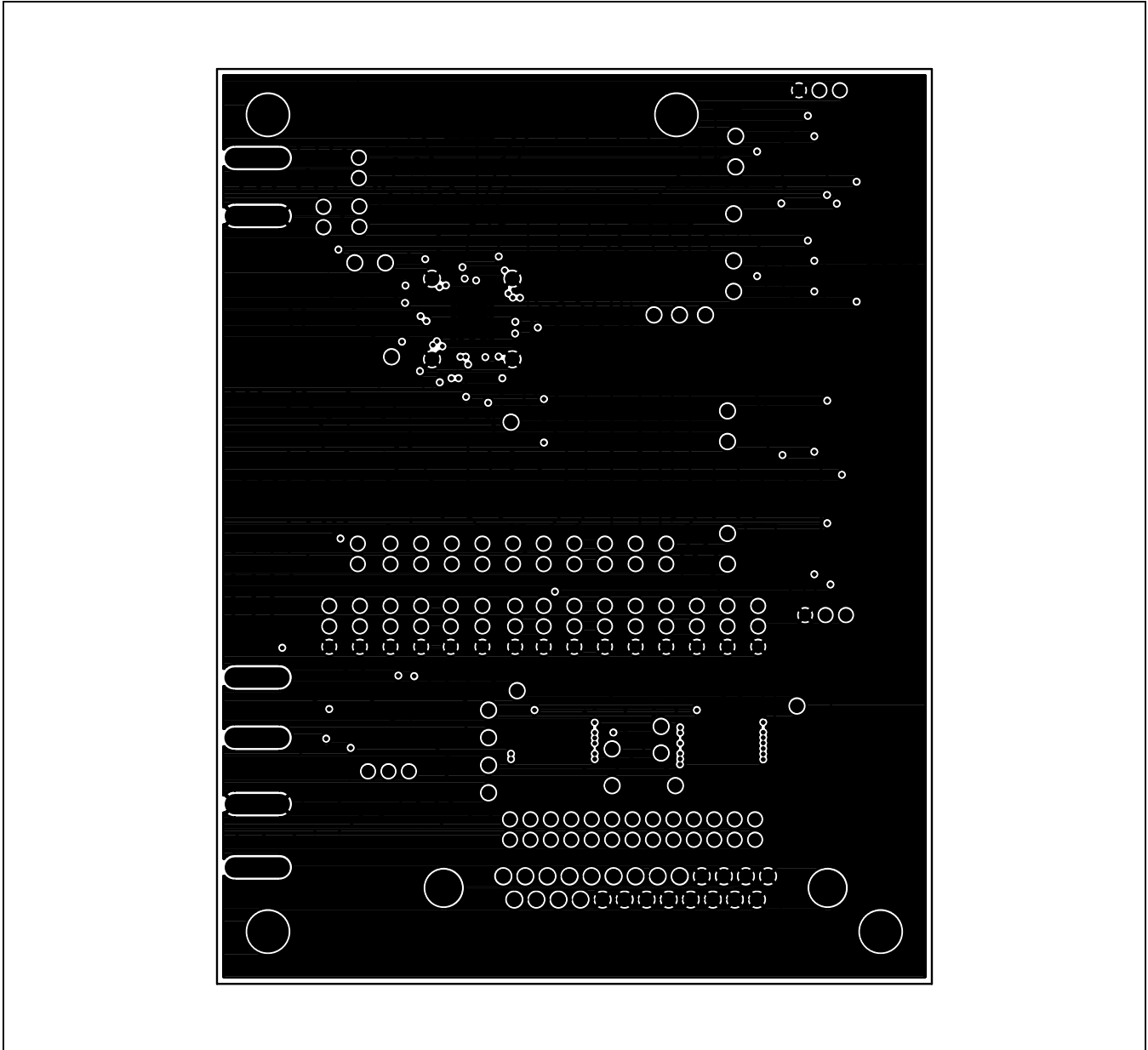
Figure 4. MAX2830 EV Kit PCB Layout—Inner Layer 2 (Ground Layer)
