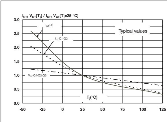
Figure 6. Relative variation of gate trigger current ( I_{GT} ) and voltage ( V_{GT} ) versus junction temperature
