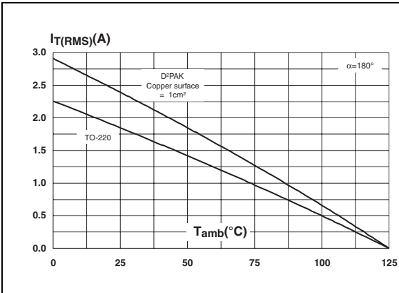
Figure 4. On-state rms current versus ambient temperature (free air convection, full cycle)
