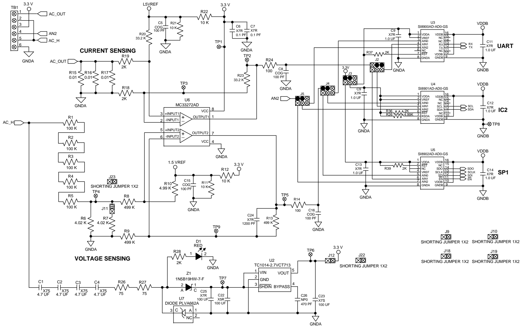
Figure 9. Measurement Circuits
