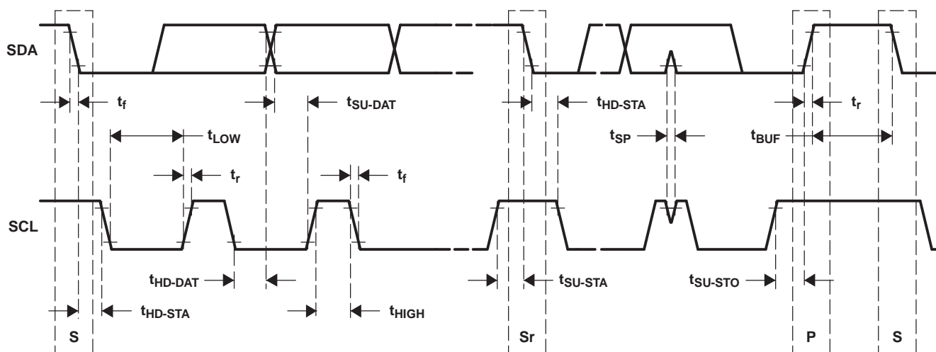
Figure 4-2. Start and Stop Conditions Timing Waveforms
