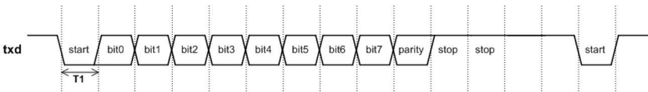
Figure 5.8 UART Timing
