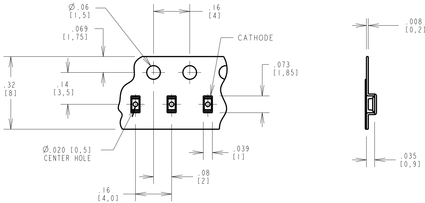
TAPE & REEL SPECIFICATION NO SCALE
