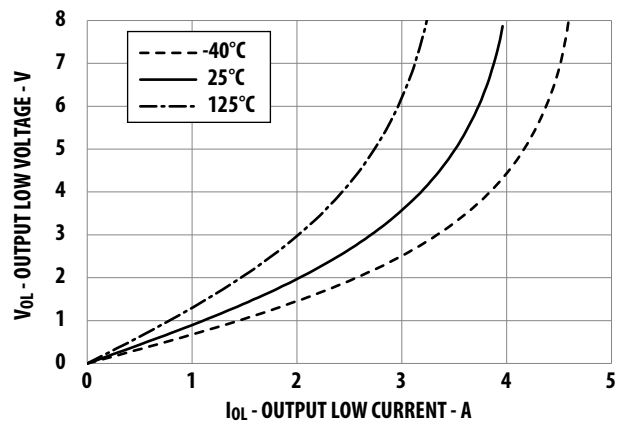
Figure 8. V_{OL} vs I_{OL}
