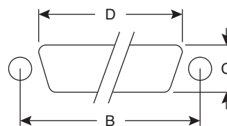
Panel Cut-Out For Front of Panel Mounting
