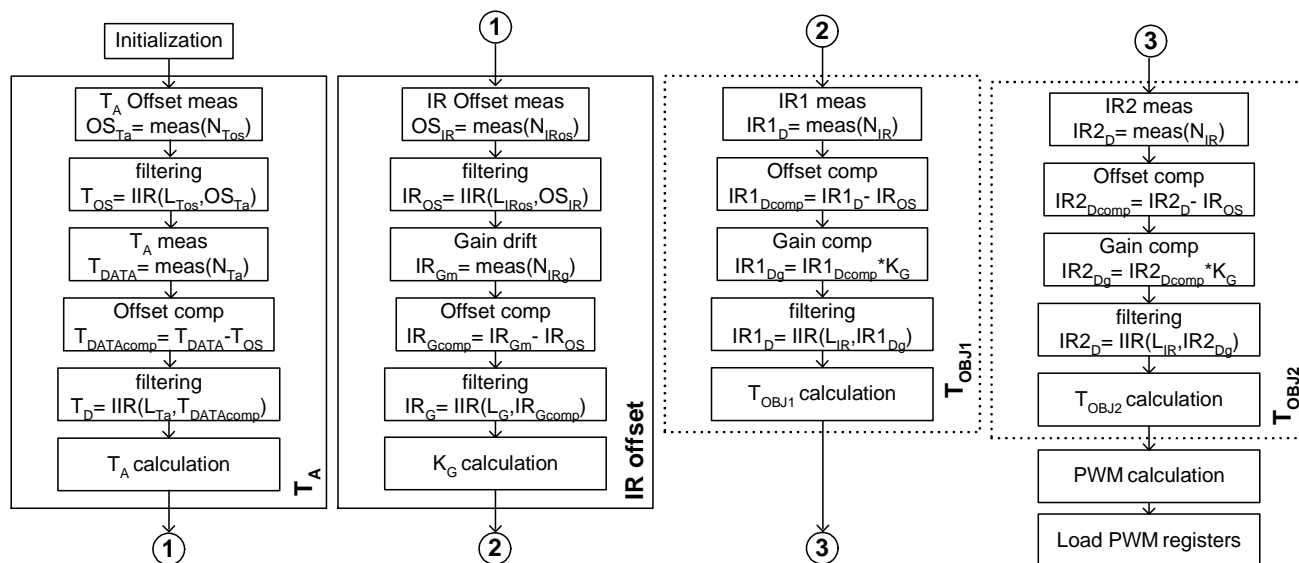
Figure 20: Software flow
