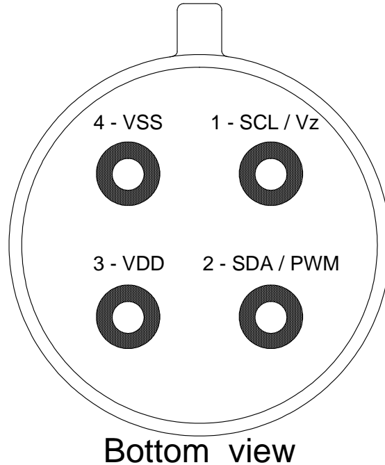
Figure 2: Pin description
