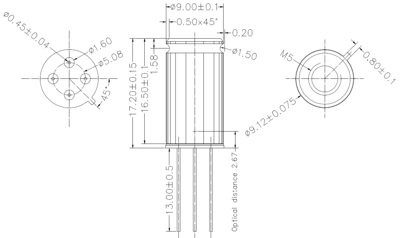
Figure 43: MLX90614xCF package
