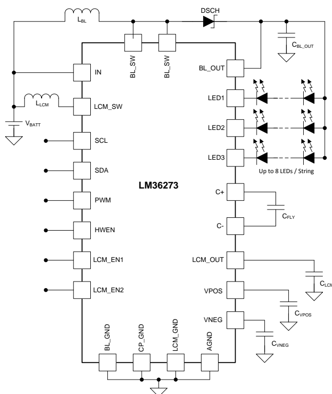
Simplified Schematic
