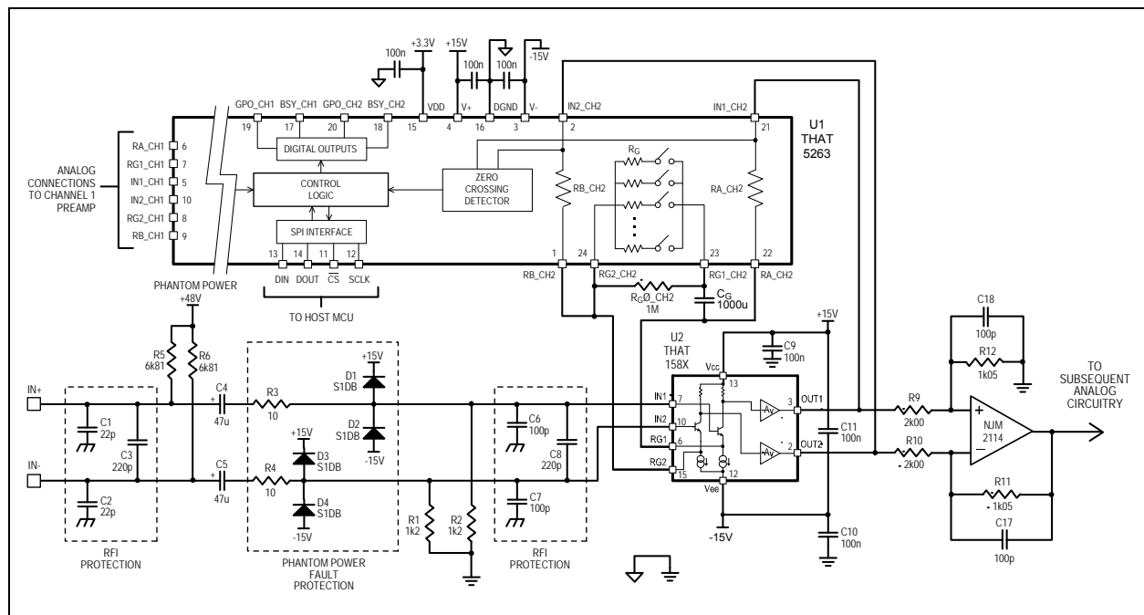
Figure 10. 5263 and 158X typical application with single-ended output.
