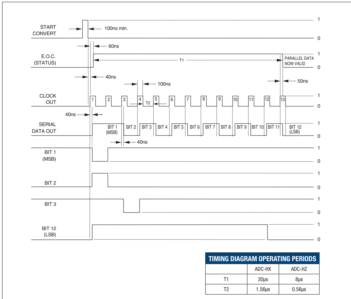
TIMING DIAGRAM FOR ADC-HX, ADC-HZ OUTPUT: 1010101010
