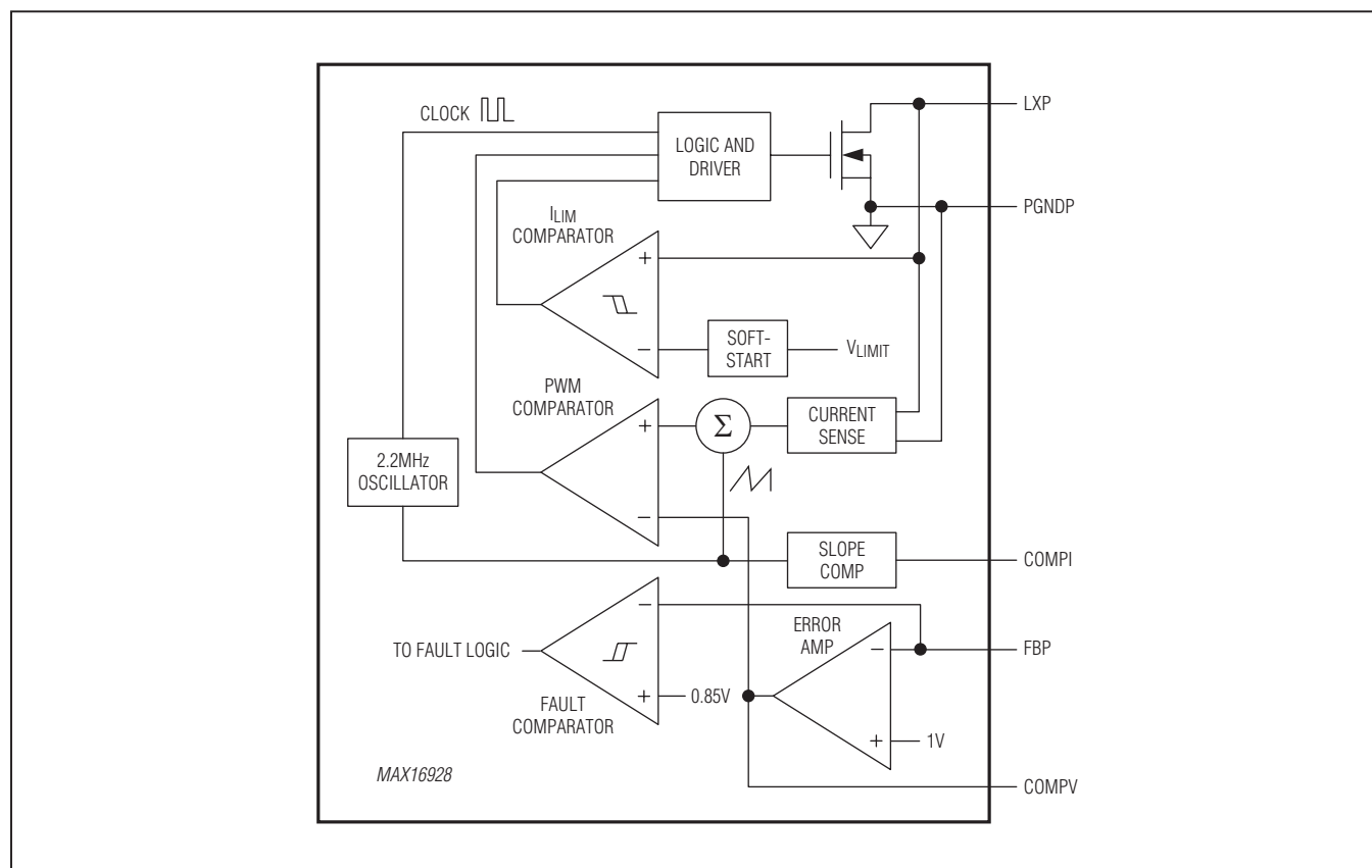
Figure 1. Boost Converter Functional Diagram
