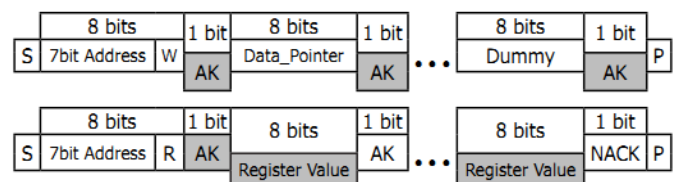
Figure 16: Typical I2C read transmission. Note: S = START, W = WRITE, R = READ, AK = acknowledge, NACK = NOT acknowledged, P = STOP. Clear boxed originate in the I2C Master and shaded boxed originate in the I2C Slave.
