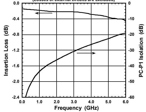
Loss, ISL vs Frequency
