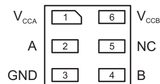
DSF PACKAGE (TOP THROUGH VIEW)
