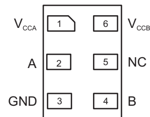
DSF PACKAGE (TOP THROUGH VIEW)
