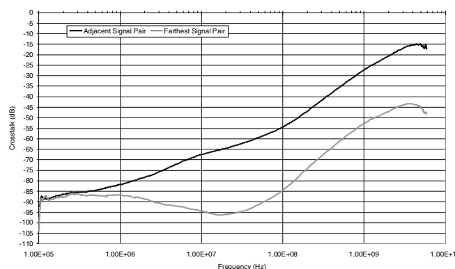
Figure 8. TPD6F003
