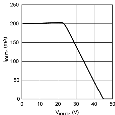
Figure 20. Over-power Protection
