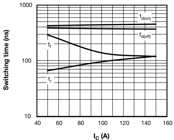
Fig. 12 - Typical IGBT Switching Time vs. I_C , T_J = 125\text{ }^\circ\text{C} , V_{CC} = 300\text{ V} , R_g = 10\text{ }\Omega , V_{GE} = 15\text{ V} , L = 500\text{ }\mu\text{H}
