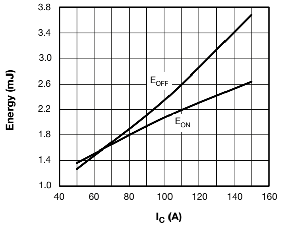
Fig. 11 - Typical Trench IGBT Energy Loss vs. I_C , T_J = 125\text{ }^\circ\text{C} , V_{CC} = 300\text{ V} , R_g = 10\text{ }\Omega , V_{GE} = 15\text{ V} , L = 500\text{ }\mu\text{H}
