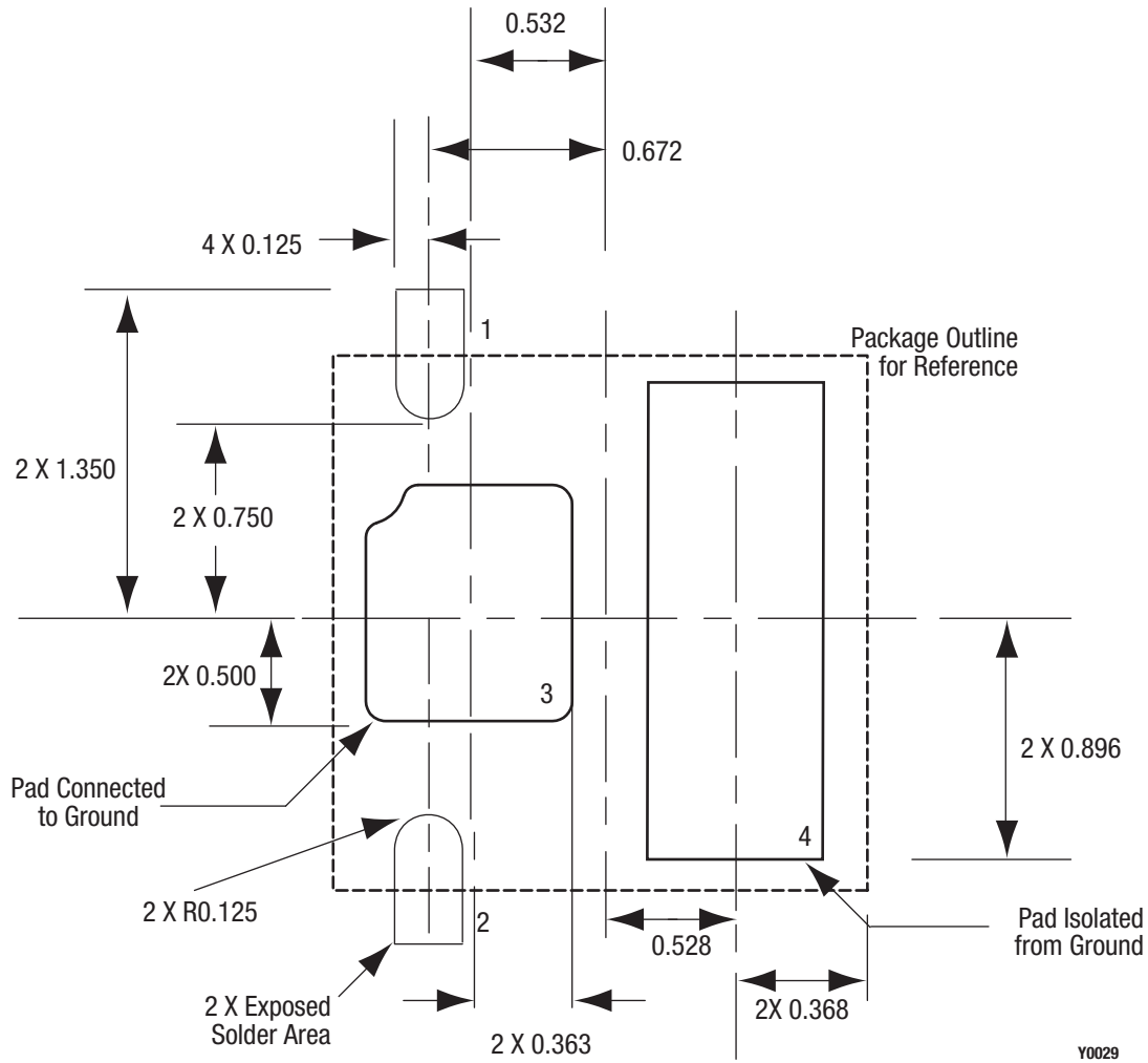
Figure 13. SKY16602-632LF PCB Layout Footprint
