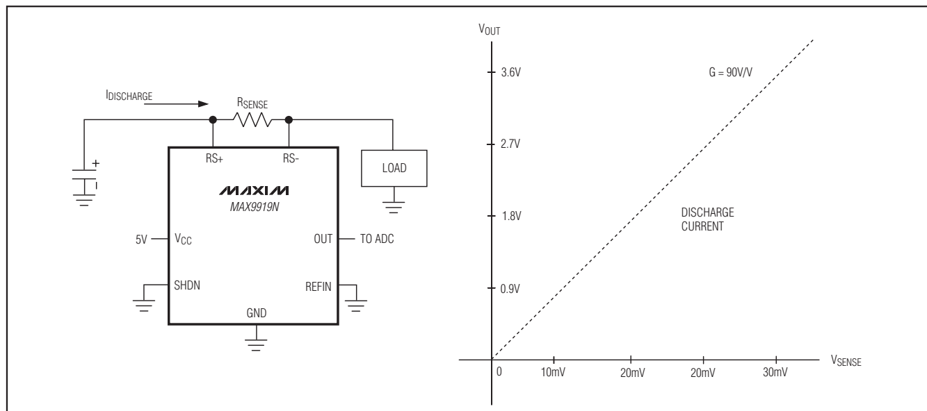
Figure 1. Unidirectional Operation
