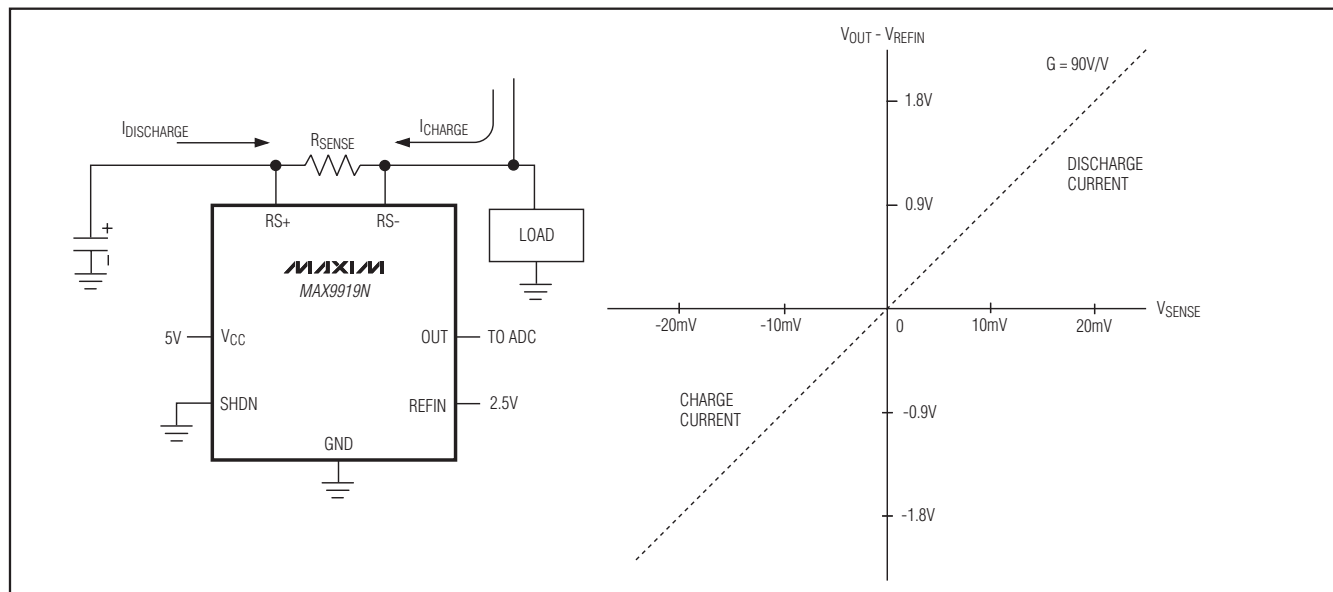
Figure 2. Bidirectional Operation
