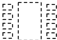
Figure 6. WSON Thermal Land Pad and Pin Pads
