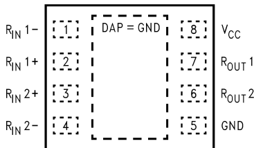
Figure 2. WSON (Top View) See Package Number NGN008A
