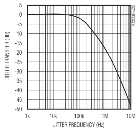
JITTER TRANSFER
