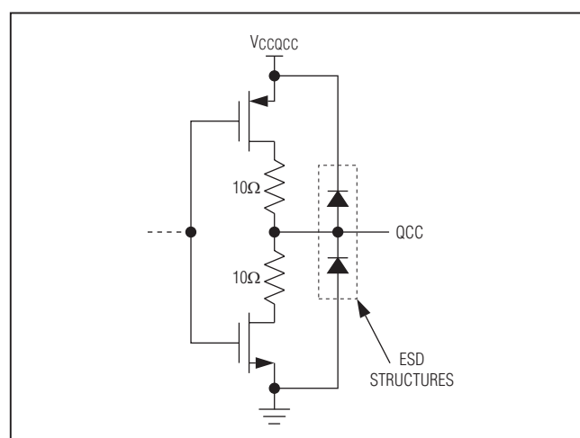
Figure 15. Equivalent LVCMOS Output Circuit
