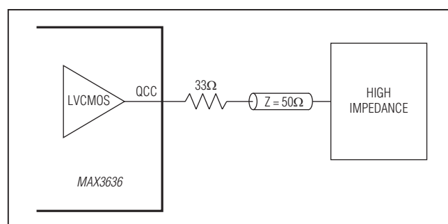
Figure 16. Interface to LVCMOS Output
