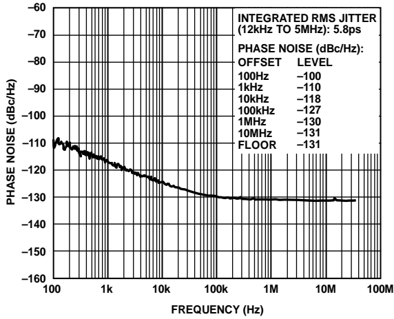
Figure 16. Phase Noise of 25 MHz, 3.3 V LVCMOS Input Clock Used
