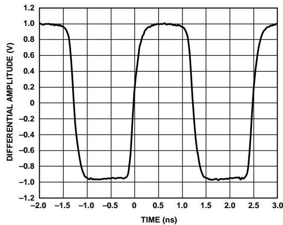
Figure 21. Output Waveform, LVPECL (400 MHz)
