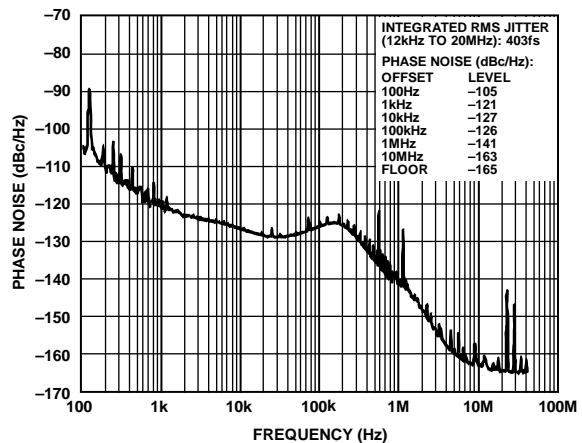
Figure 9. Absolute Phase Noise (Output Driver = LVPECL), f_R = 49.152 MHz Crystal, f_{OUT} = 174.703 MHz on Both PLLs
