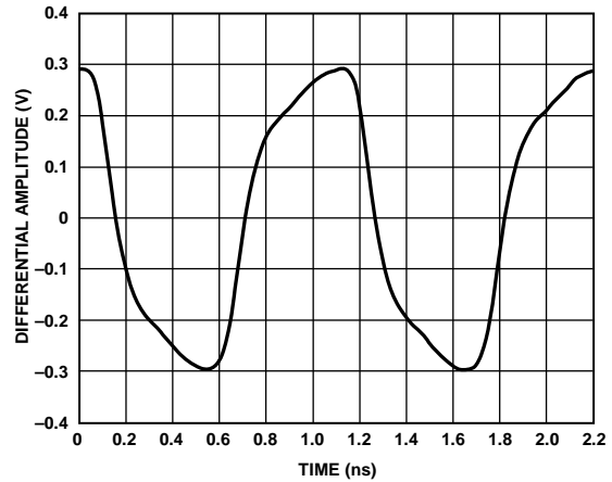
Figure 20. Output Waveform, LVDS (900 MHz)
