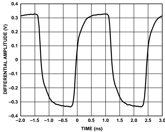
Figure 17. Output Waveform, LVDS (400 MHz)
