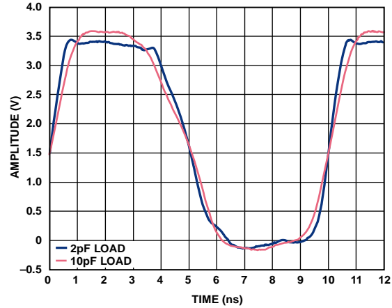
Figure 19. Output Waveform, 3.3 V CMOS (100 MHz)
