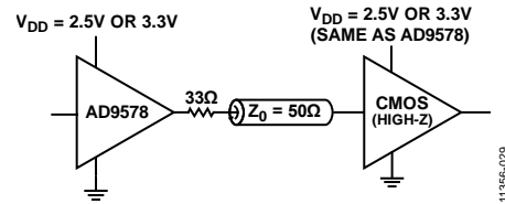
Figure 30. DC-Coupled LVCMOS Termination
