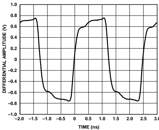
Figure 18. Output Waveform, HCSSL (400 MHz)
