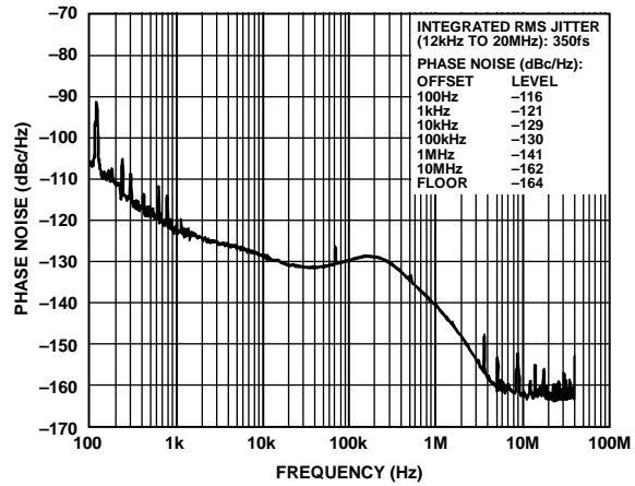
Figure 7. Absolute Phase Noise (Output Driver = LVDS), f_R = 49.152 MHz Crystal, f_{OUT} = 156.25 MHz on Both PLLs
