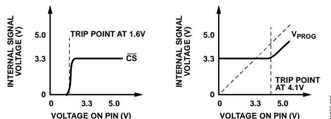
Figure 35. \overline{CS} Pin Function
