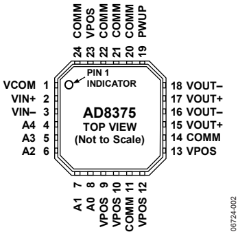
Figure 3. 24-Lead LFCSP
