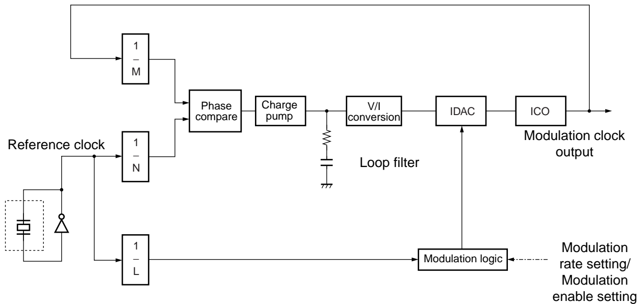
MB88151 PLL block
