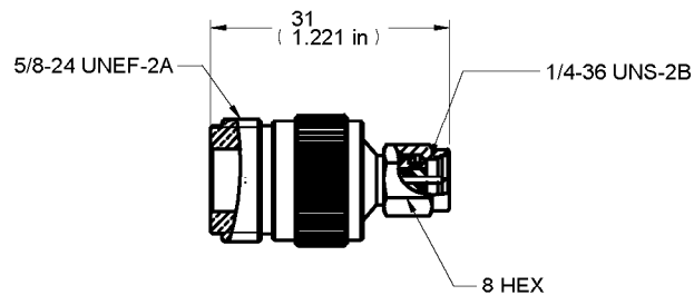
DIM OUTLINE
