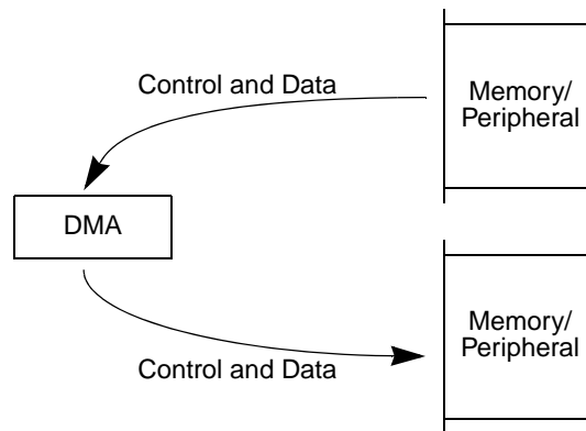
Figure 16-3. Dual-Address Transfer
