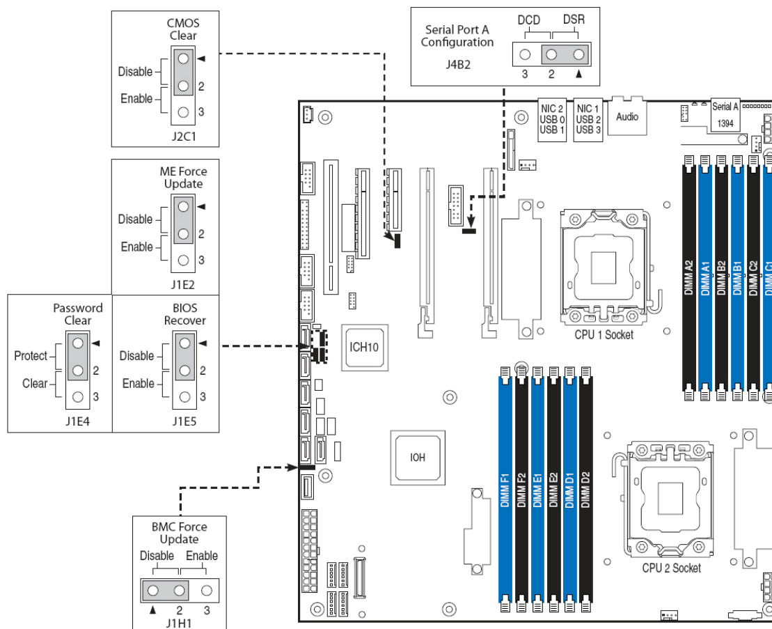
Figure 45. Jumper Blocks
