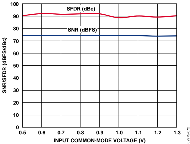
Figure 43. SNR/SFDR vs. Input Common-Mode Voltage, f_{IN} = 70 \text{ MHz} , f_s = 125 \text{ MSPS}
