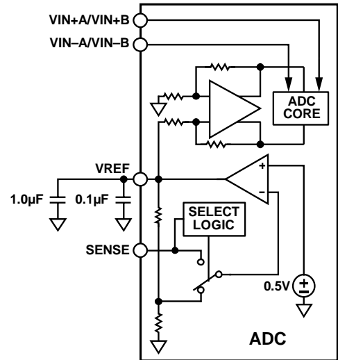
Figure 49. Internal Reference Configuration
