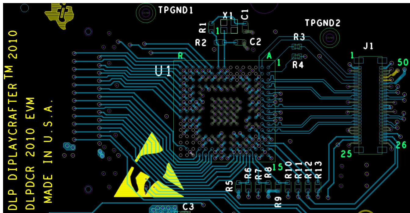
Figure 26. Layout Recommendation
