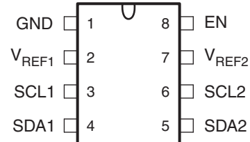
DCU PACKAGE (TOP VIEW)
