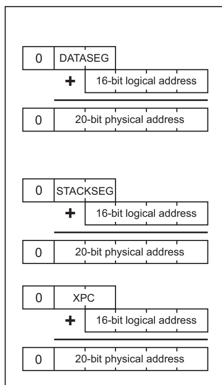
Figure 5-3. MMU Operation
