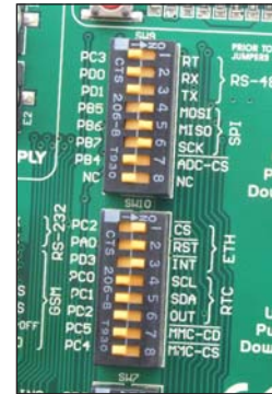
Figure 8-2: DIP switches SW9 and SW10
