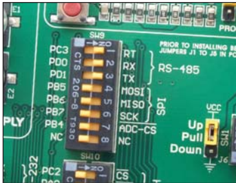
Figure 5-3: DIP switch SW9
