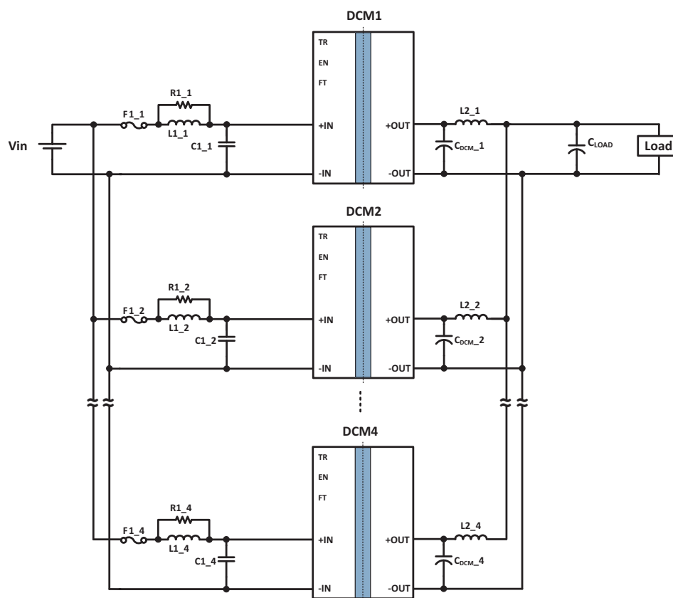
Typical Application 1: MDCM28AP150M320A50 in an array of four units
