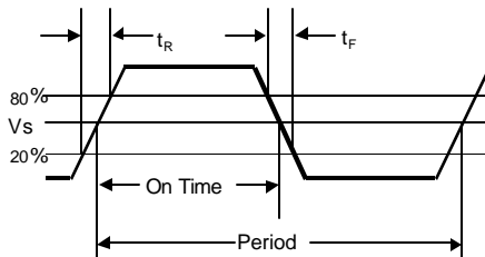
Figure 7. Output Waveform
