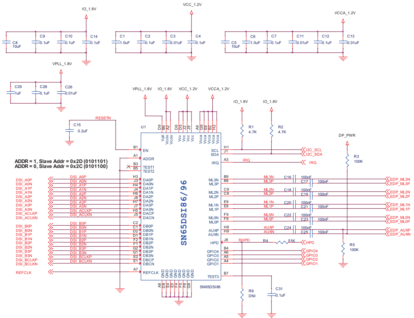
Figure 18. Typical Implementation
