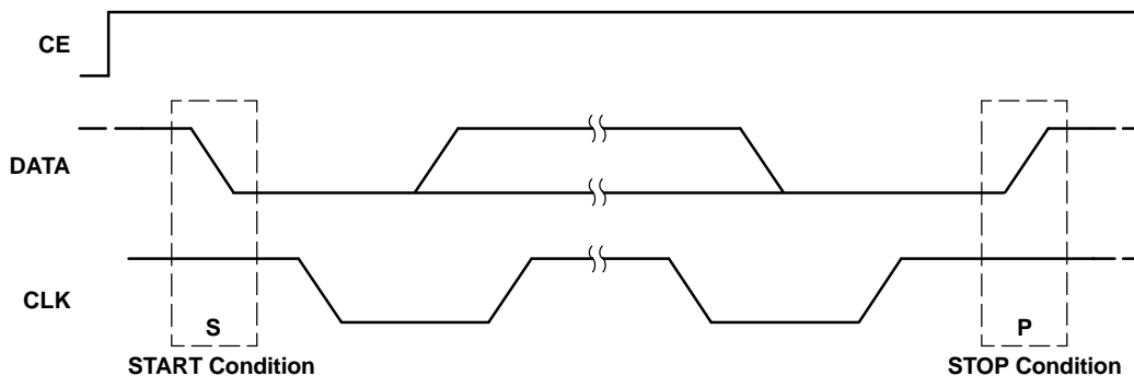
Figure 40. START and STOP Conditions
