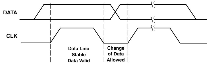
Figure 39. Bit Transfer on the Serial Interface
