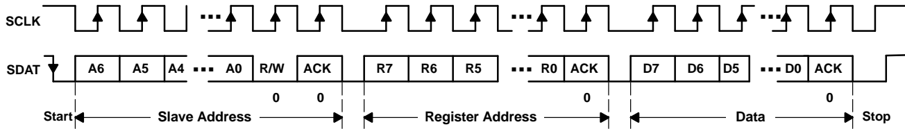
Figure 41. Serial Interface WRITE to TPS65014 Device
