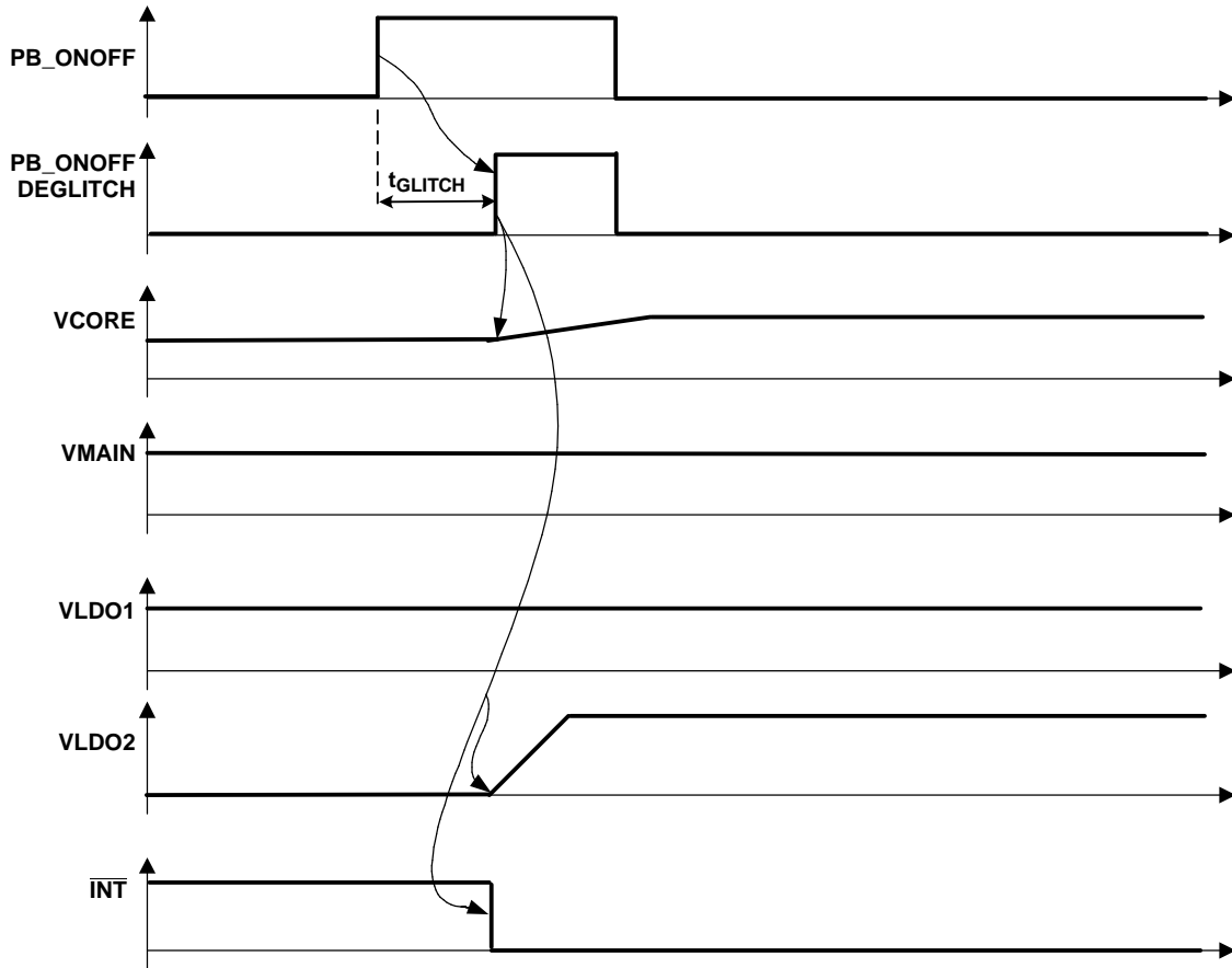
Figure 36. State 3 to State 2 Transition. PB_ONOFF Activated (See Interrupt Management Section for \overline{\text{INT}} Behavior)
