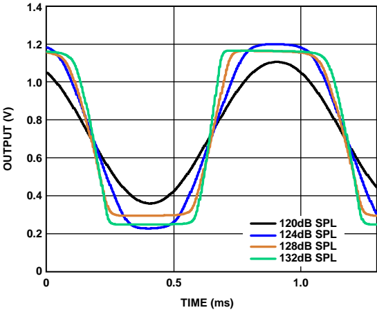
Figure 8. Clipping Characteristics
