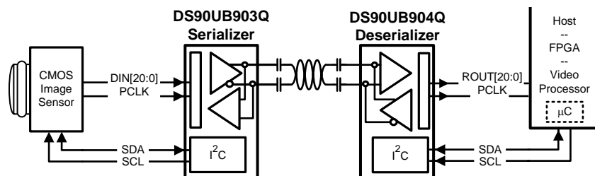
Figure 30. Typical Camera System Diagram
