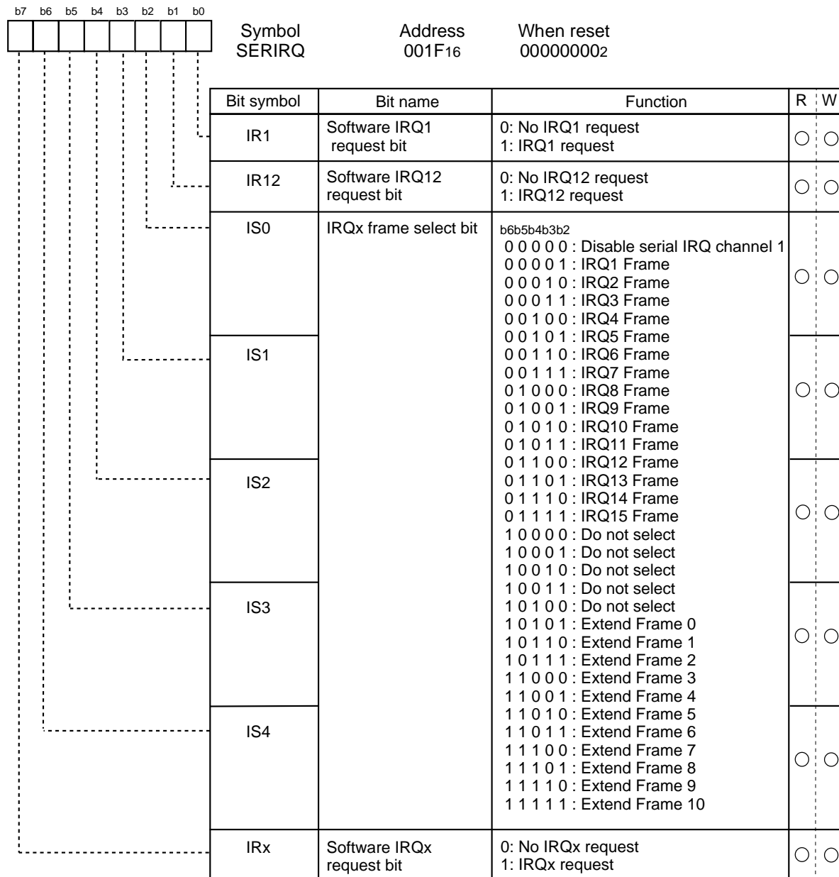
Fig. 53 Structure of serialized IRQ request register
