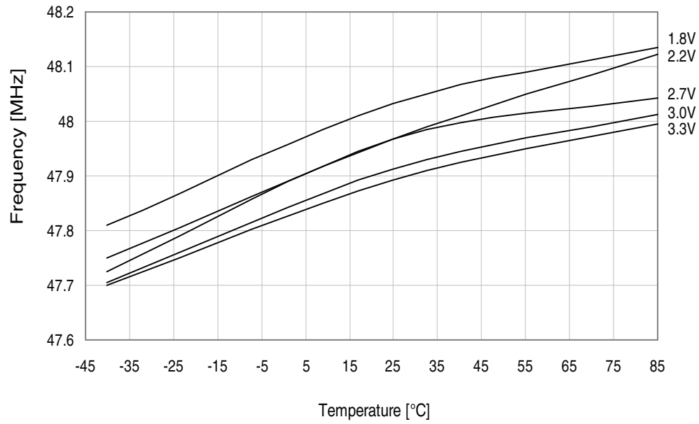
Figure 36-64. 48MHz internal oscillator frequency vs. temperature.
