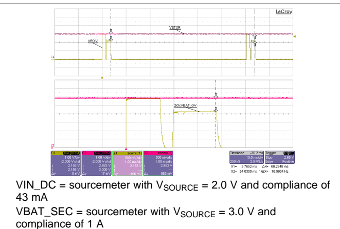
Figure 38. VRDIV Waveform
