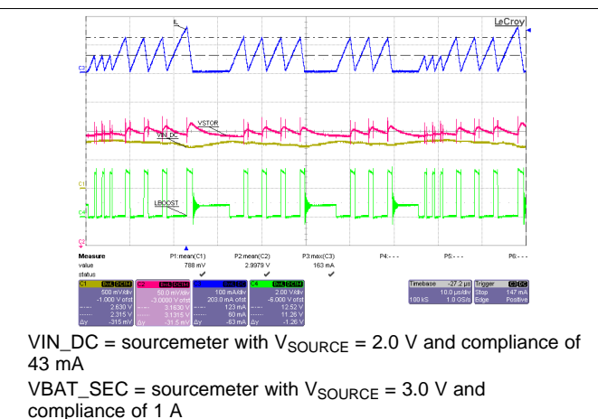
Figure 36. Boost Charger Operational Waveforms
