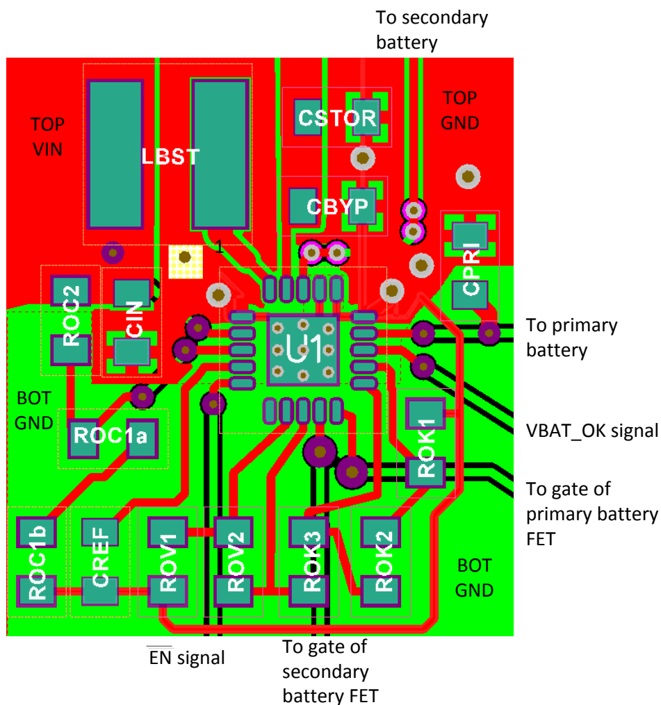
Figure 40. Layout Example
