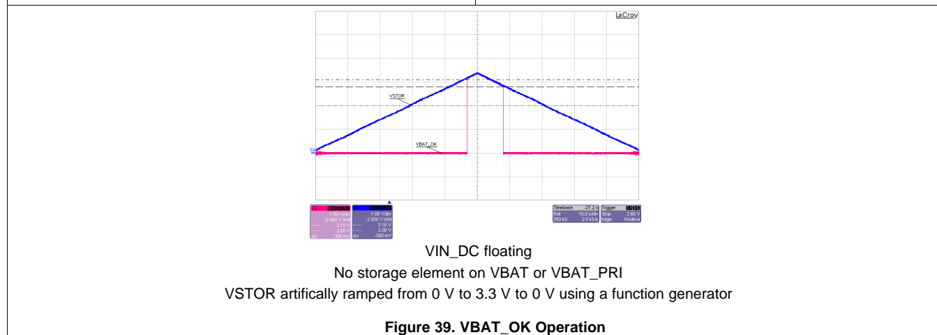
Figure 39. VBAT_OK Operation
