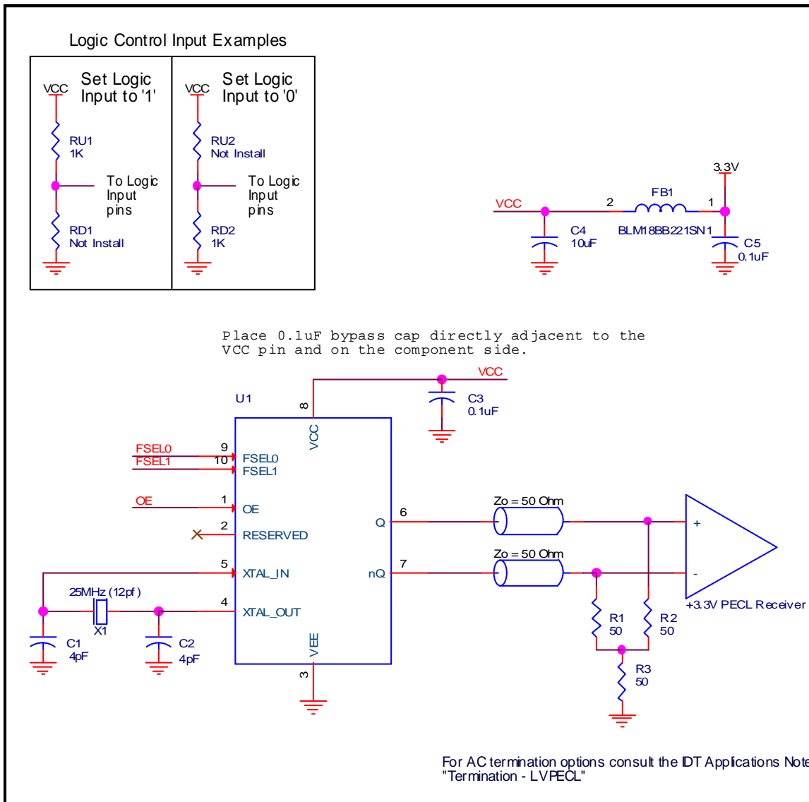
Figure 5. IDT83PN15639I Application Schematic
