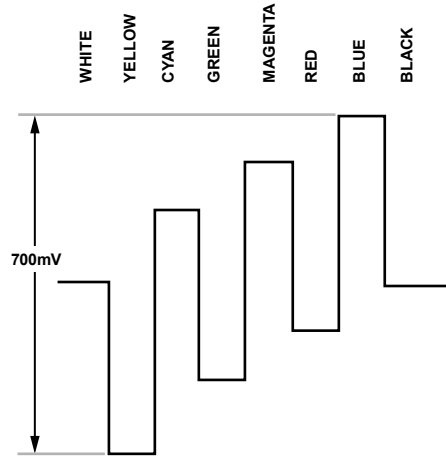
Figure 119. Pb Levels—PAL
