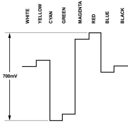
Figure 118. Pr Levels—PAL
