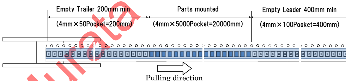
Figure 16 Pulling direction and Trailer/Leader
