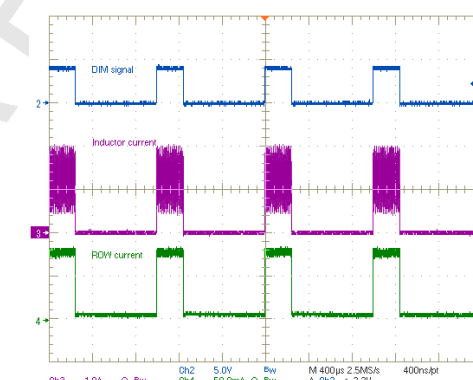
Figure 27. Dimming waveforms ( F_{DIM} = 1 kHz)
